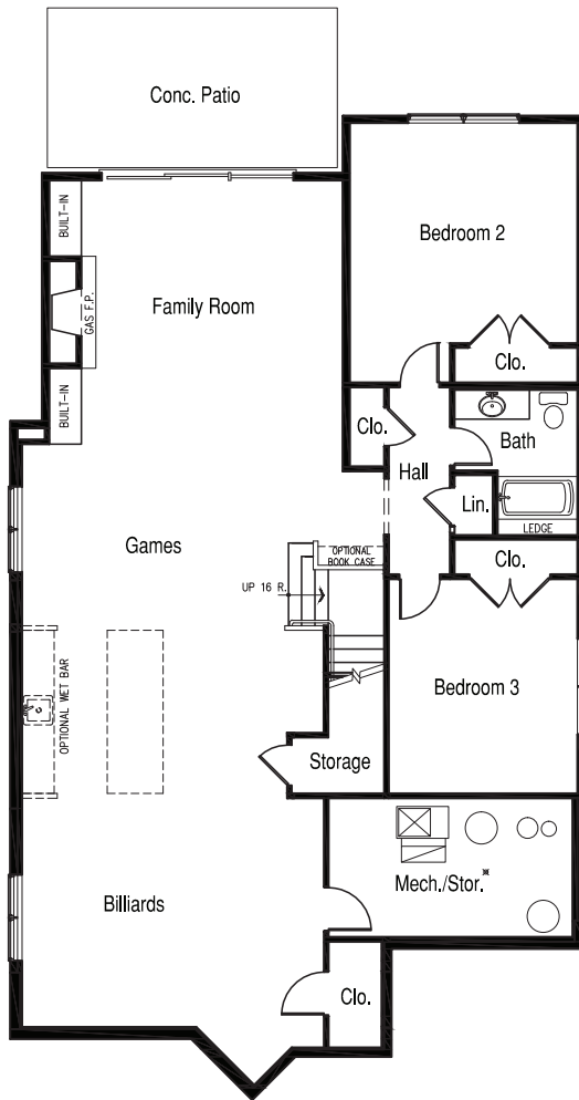
LOWER LEVEL FLOOR PLAN
