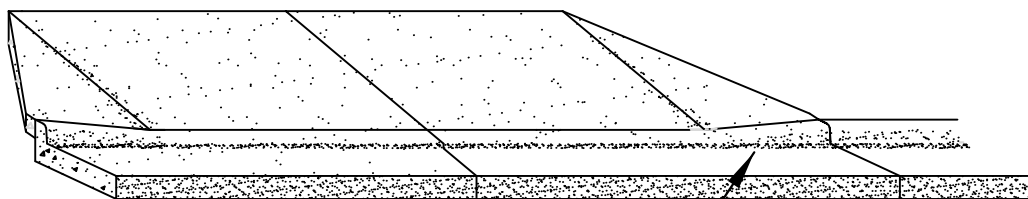
DROP CURB AT DRIVEWAYS
